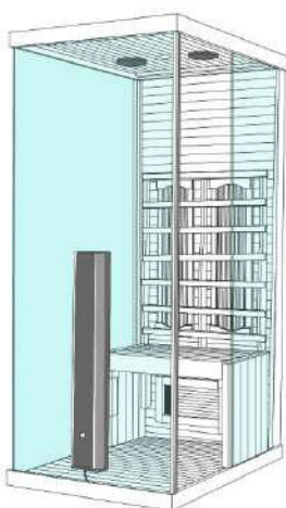
(9) Put the bench and use the screws 4x50mm to fix the bench (10) Install the hinges
